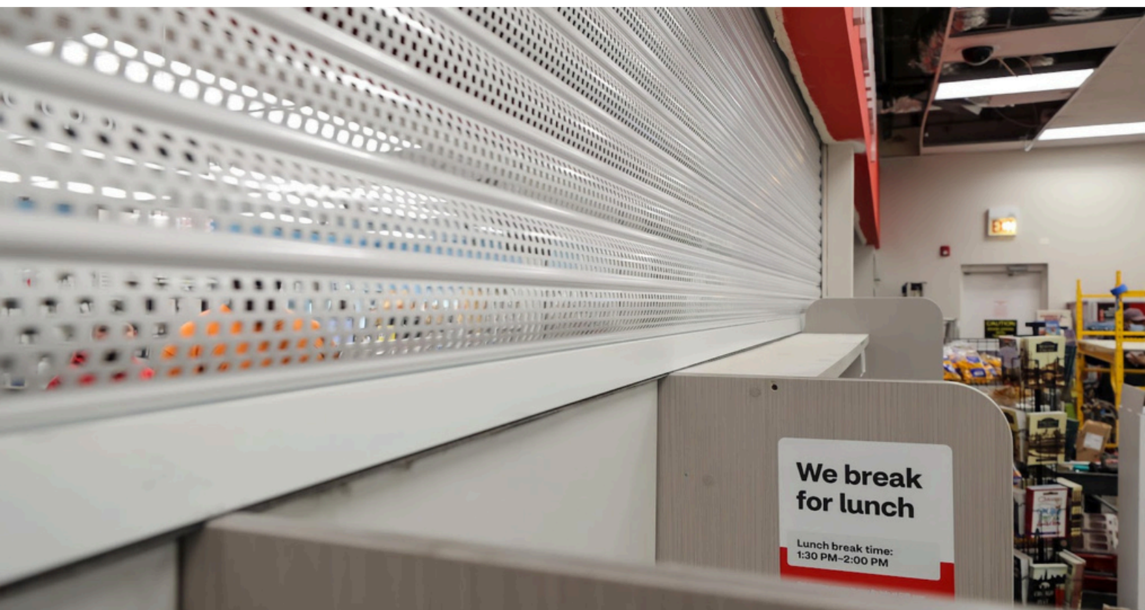
AL8 protects a pharmacy counter while providing views for both customers and staff.
